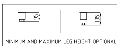
MINIMUM AND MAXIMUM HEIGHT STANDARD LEG
