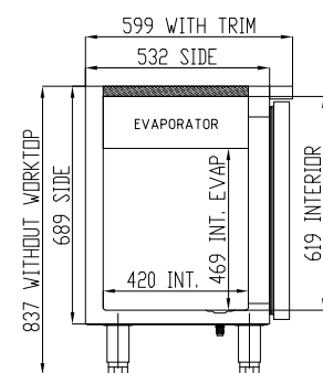
WITHOUT WORKTOP
