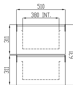
DRAWERS KIT 1/2 + 1/2
