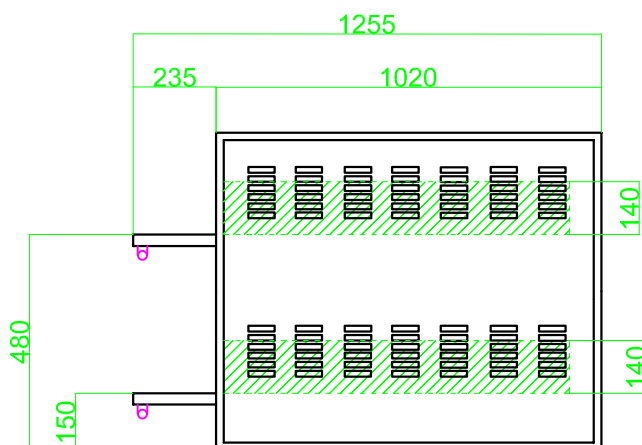
VISTA LATERALE Side view
