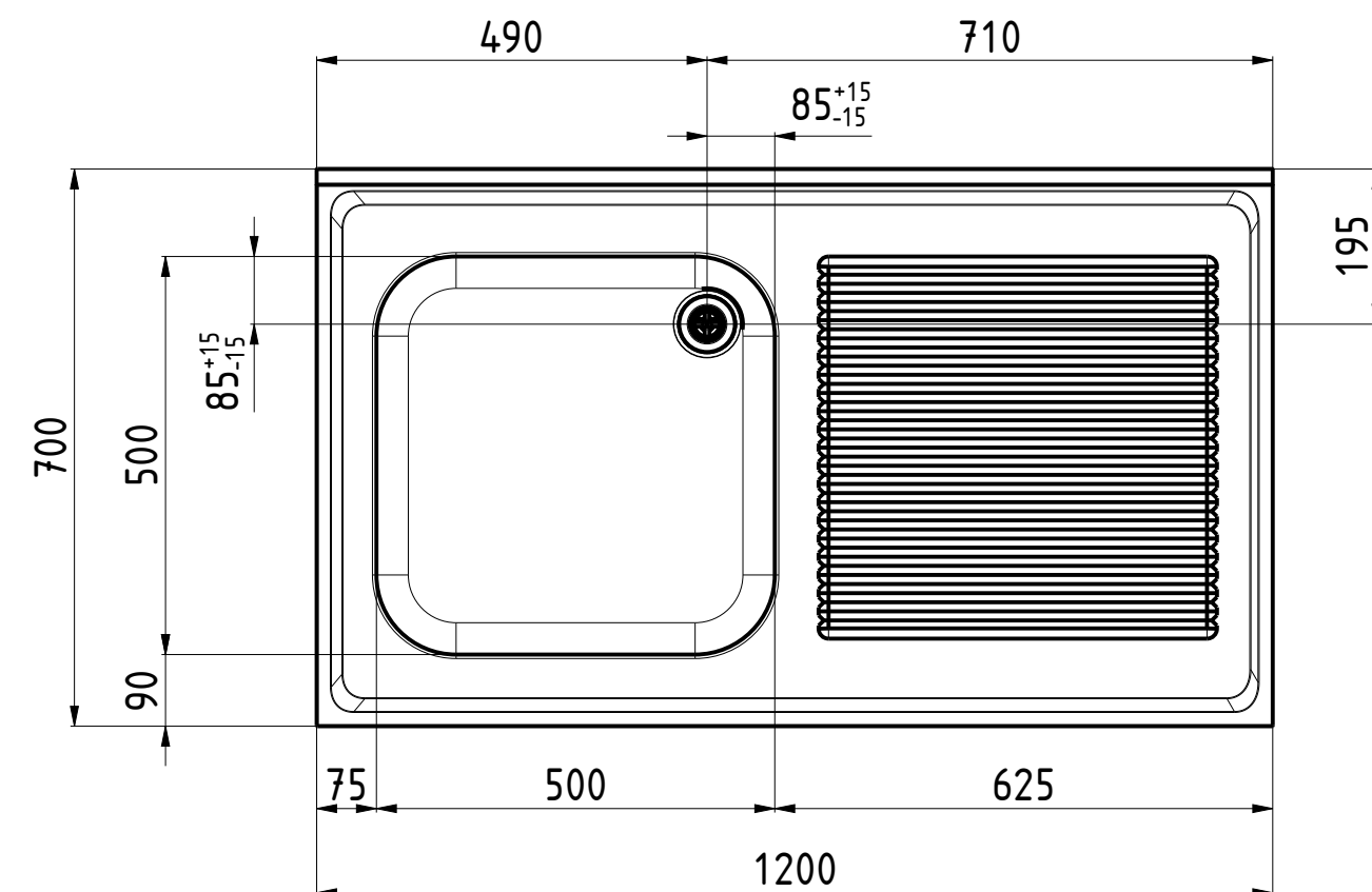
FRONT VIEW 1:10
