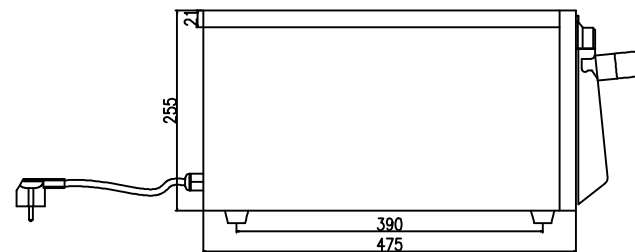
2- Side view
