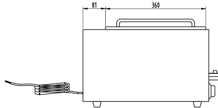
2- Side view
