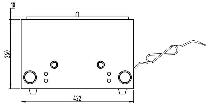
1- Front view
