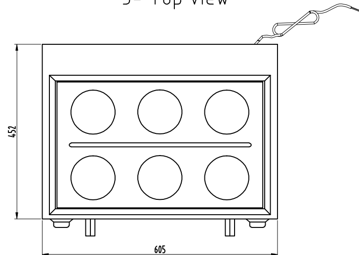
3- Top view
