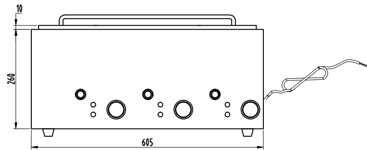
1- Front view
