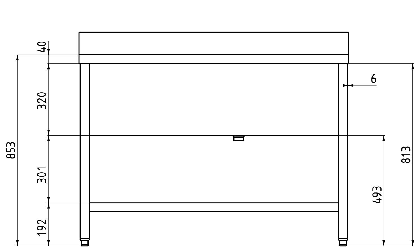
FRONT VIEW 1:10
