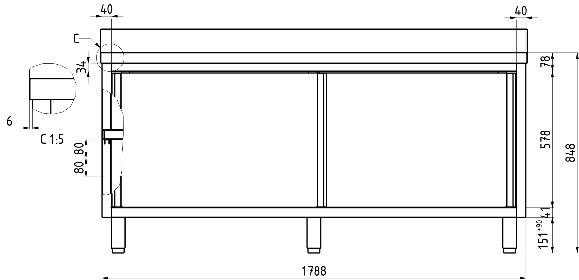
FRONT VIEW C-C 1:10
