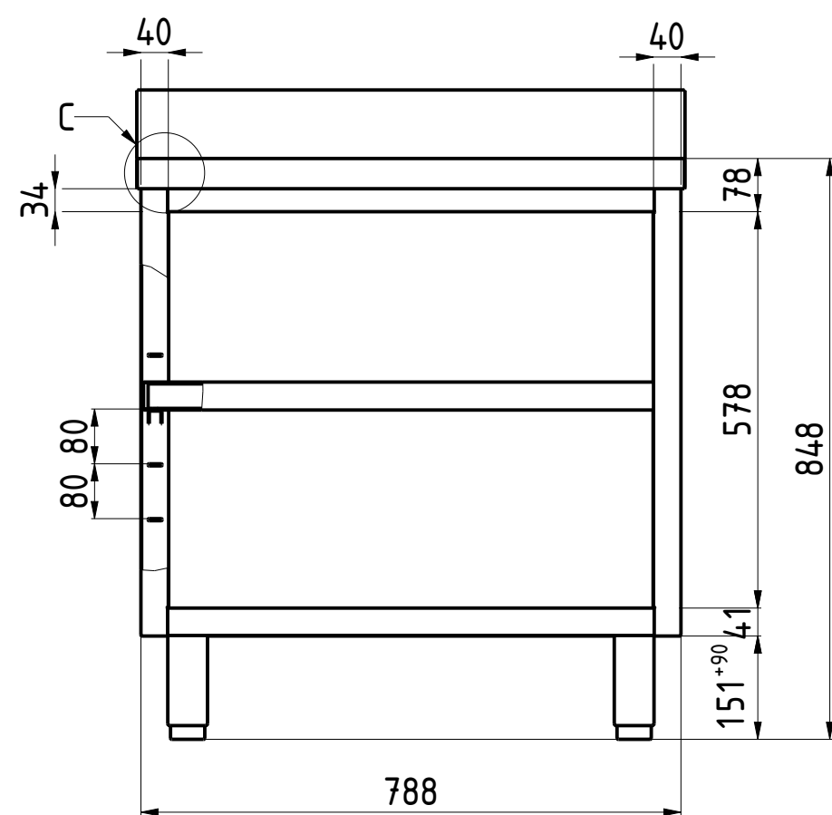
FRONT VIEW C-C 1:10
