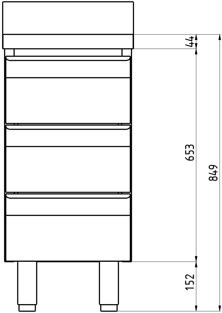
FRONT VIEW 3:20
