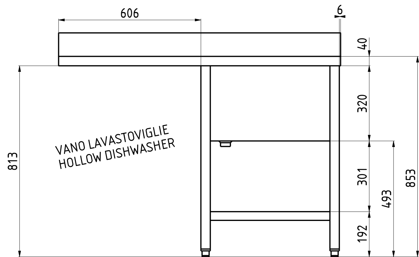
FRONT VIEW 1:10
