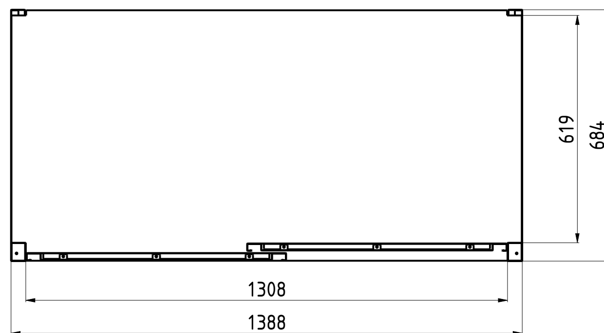
INTERNAL DIM D-D
