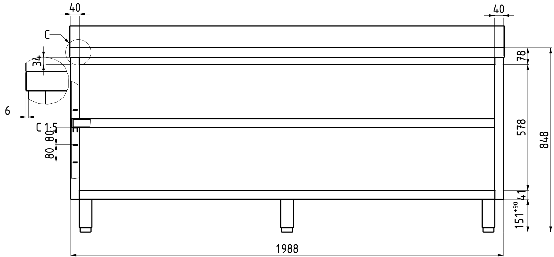
FRONT VIEW C-C 1:10
