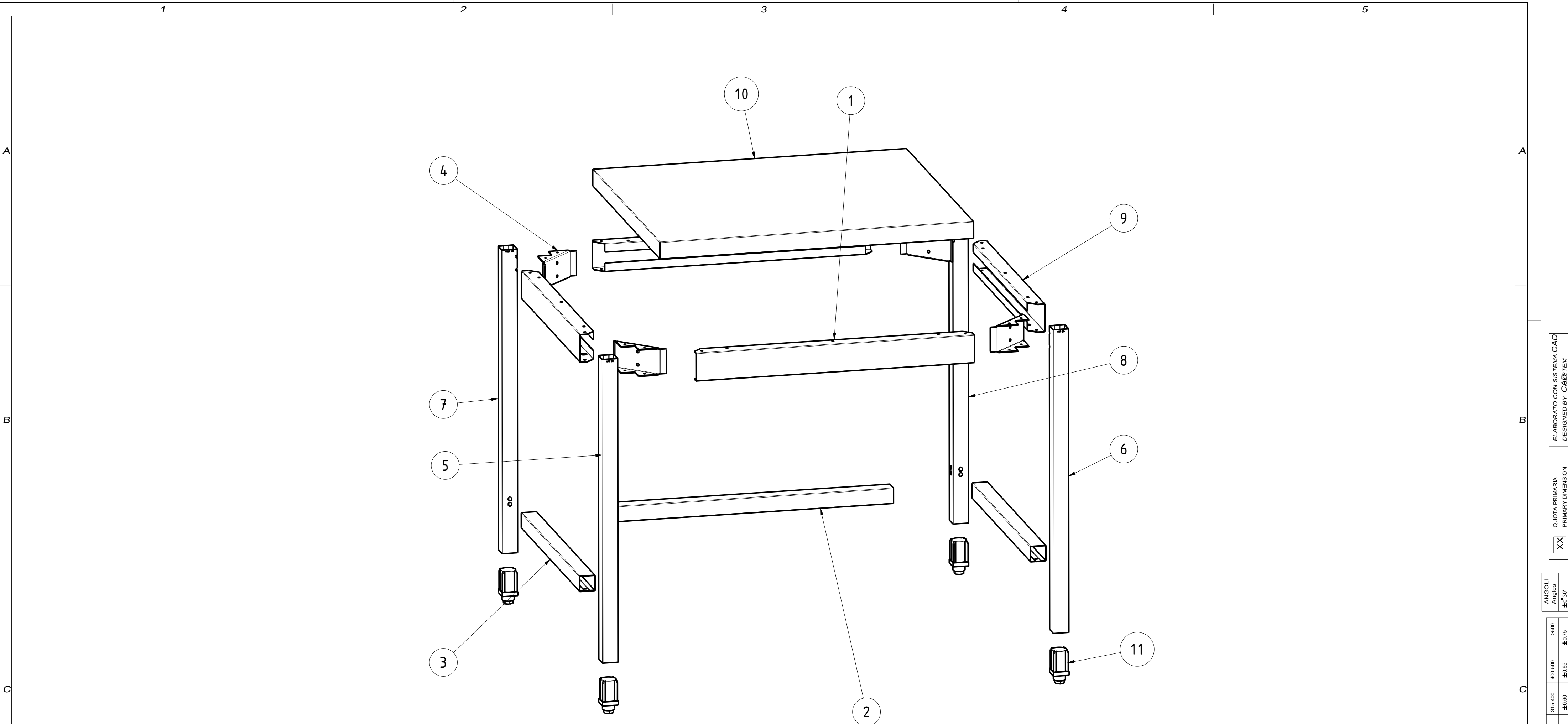
EXPLODED VIEW 3:20
