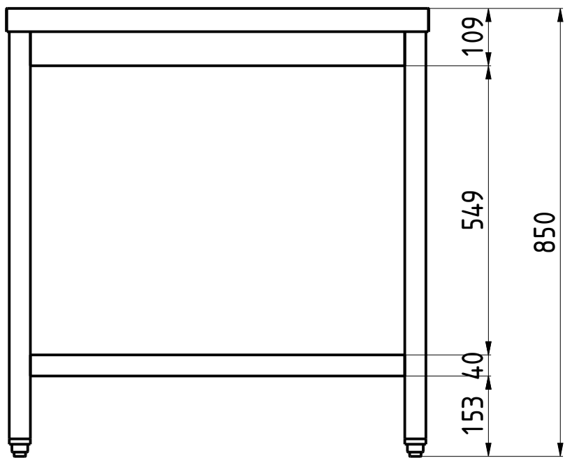
FRONT VIEW 1:10
