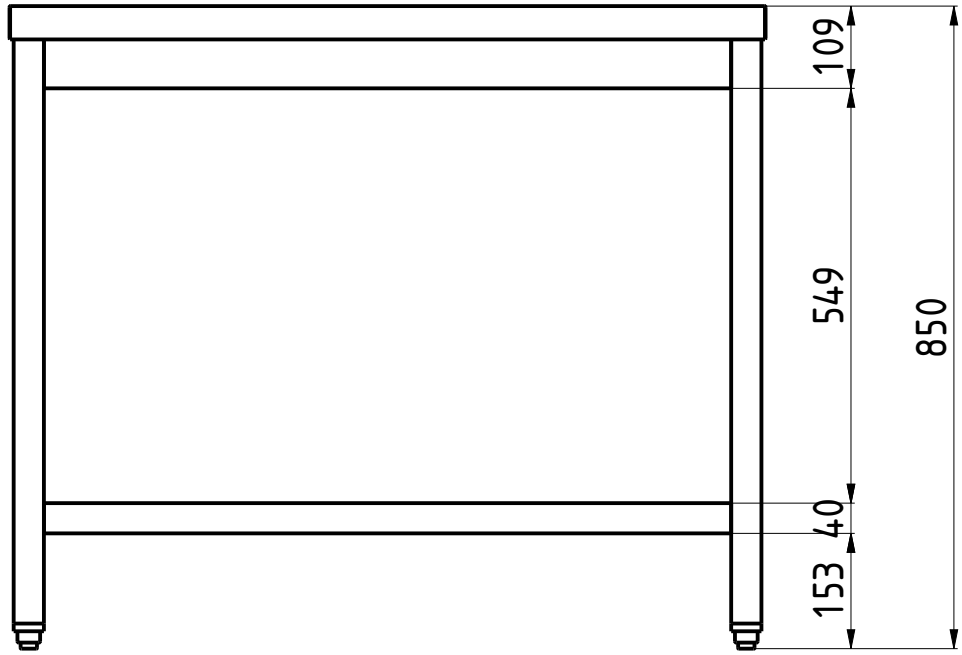
FRONT VIEW 1:10
