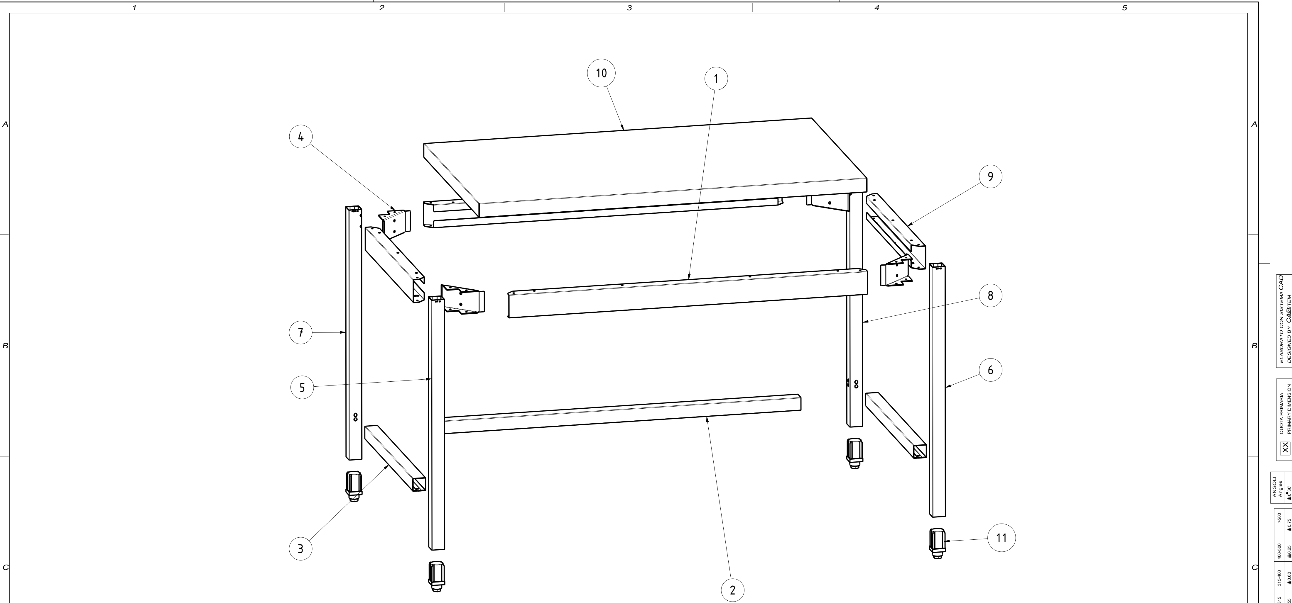
EXPLODED VIEW 3:20
