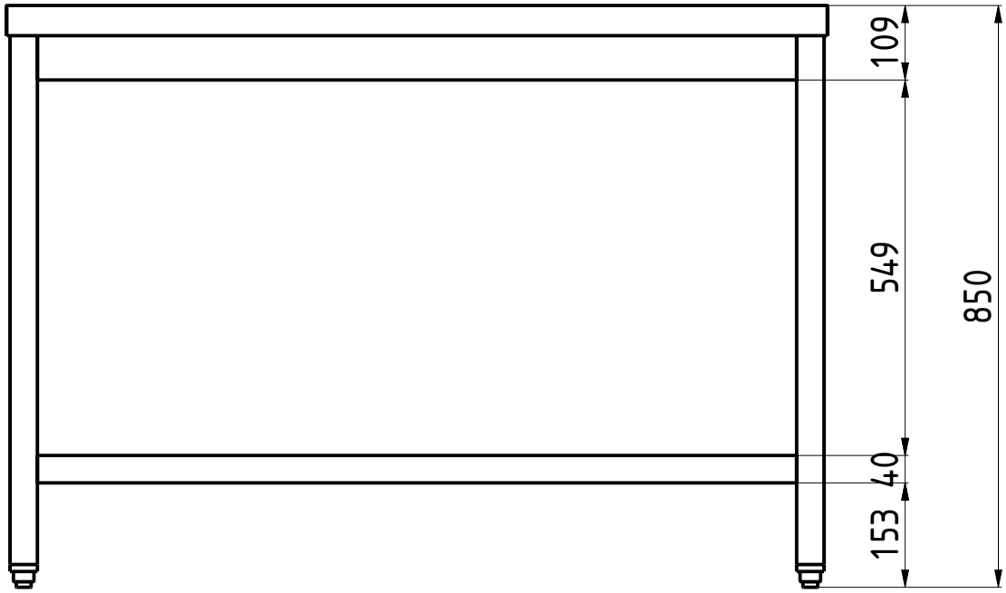
FRONT VIEW 1:10
