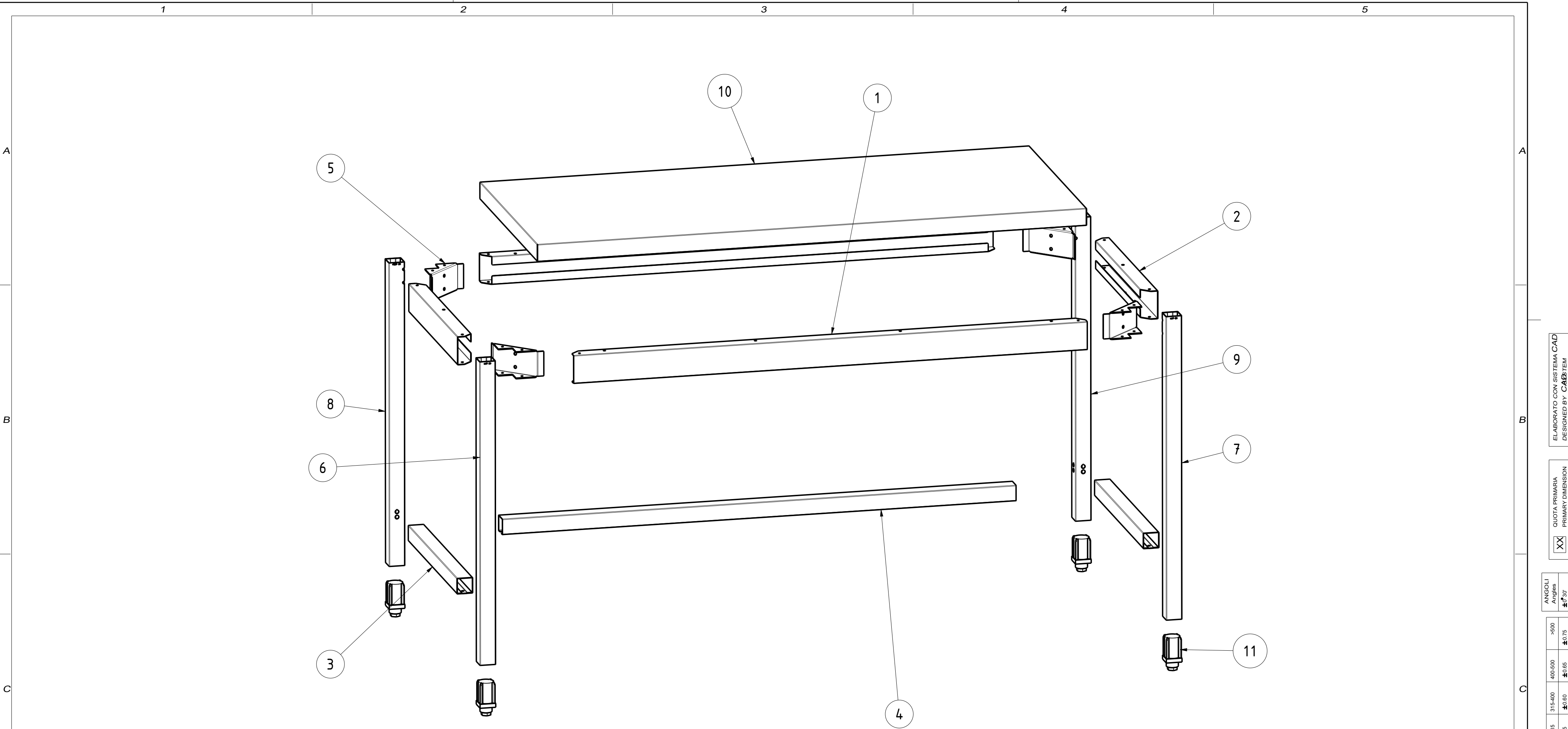
EXPLODED VIEW 3:20
