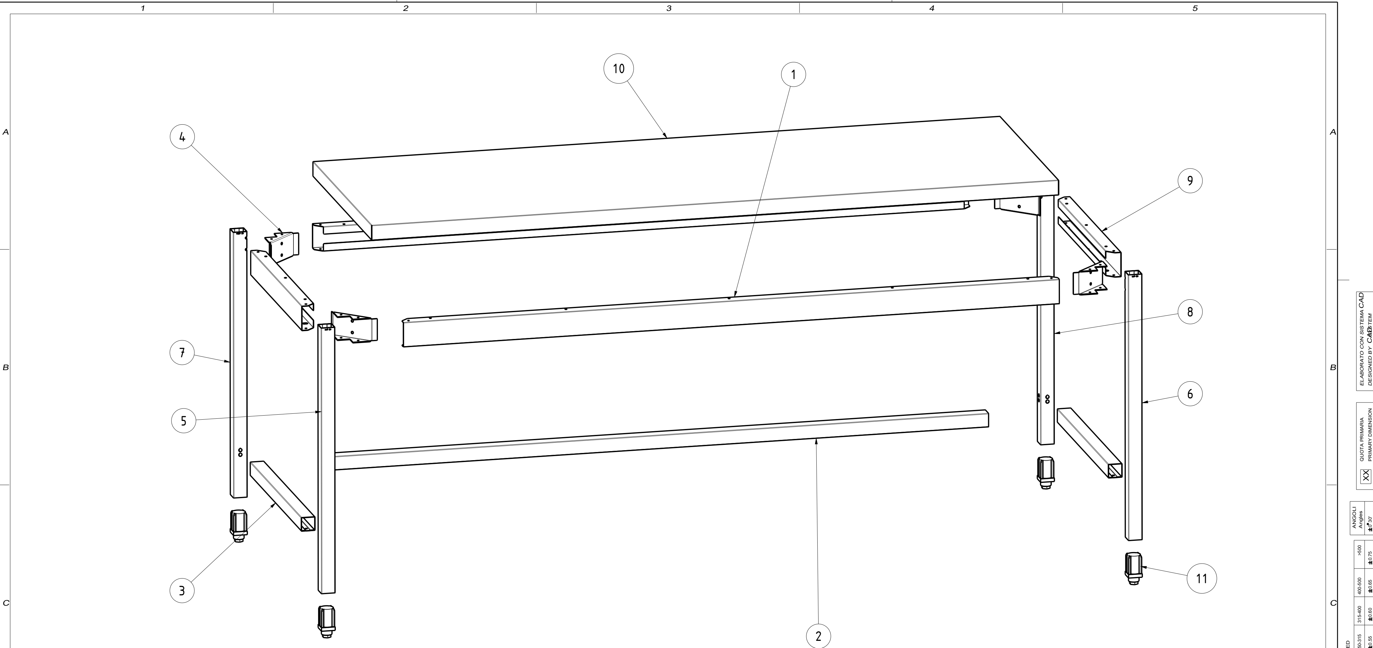
EXPLODED VIEW 3:20
