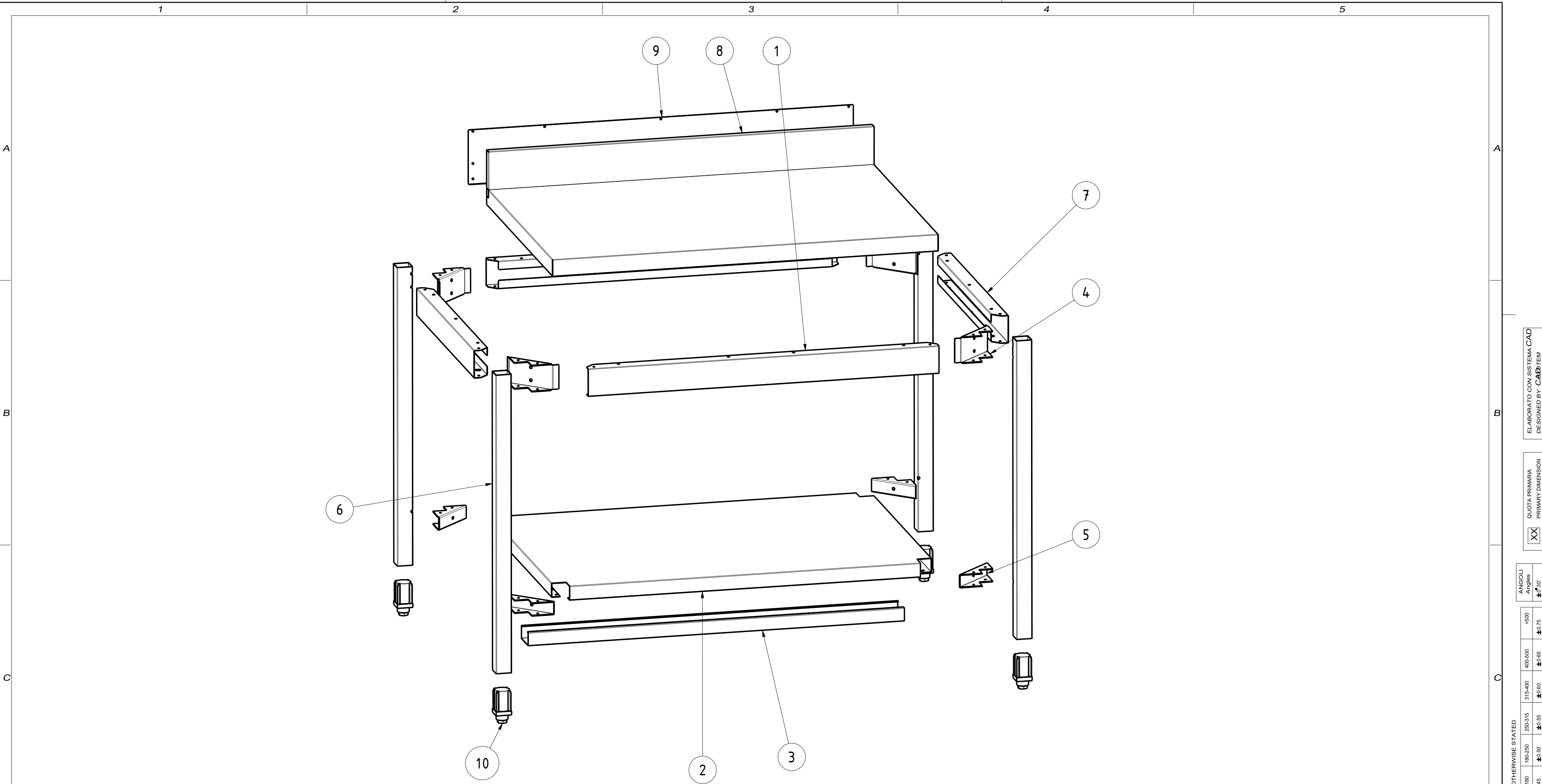
EXPLODED VIEW 3:20
