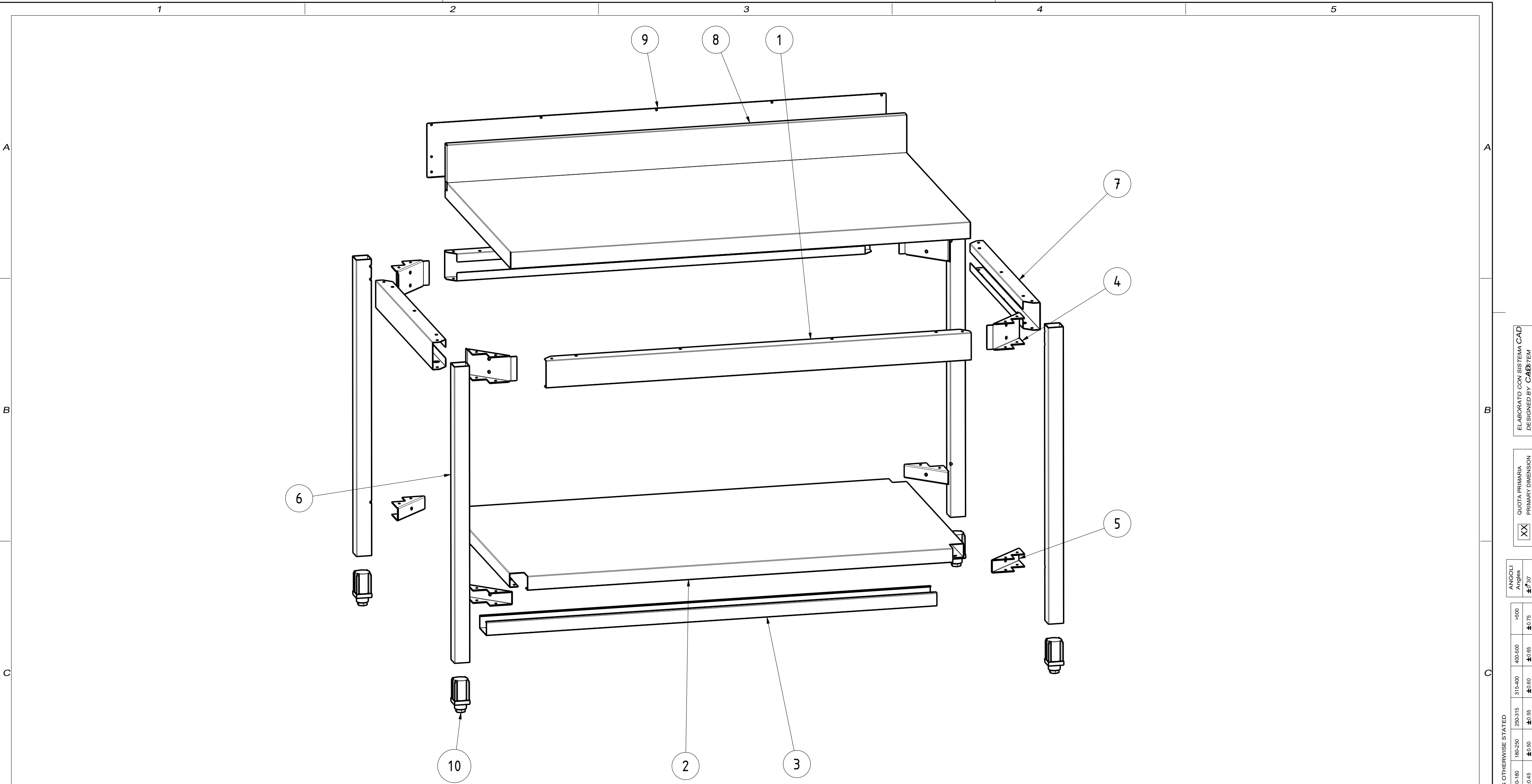
EXPLODED VIEW 3:20
