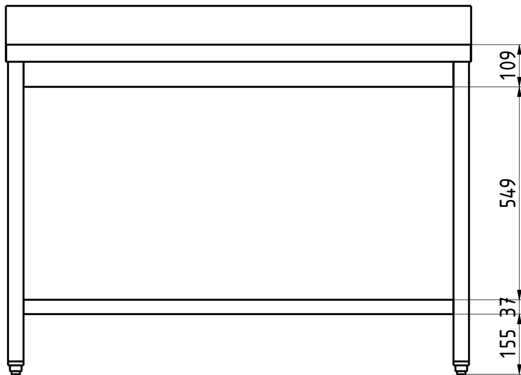
FRONT VIEW 1:10
