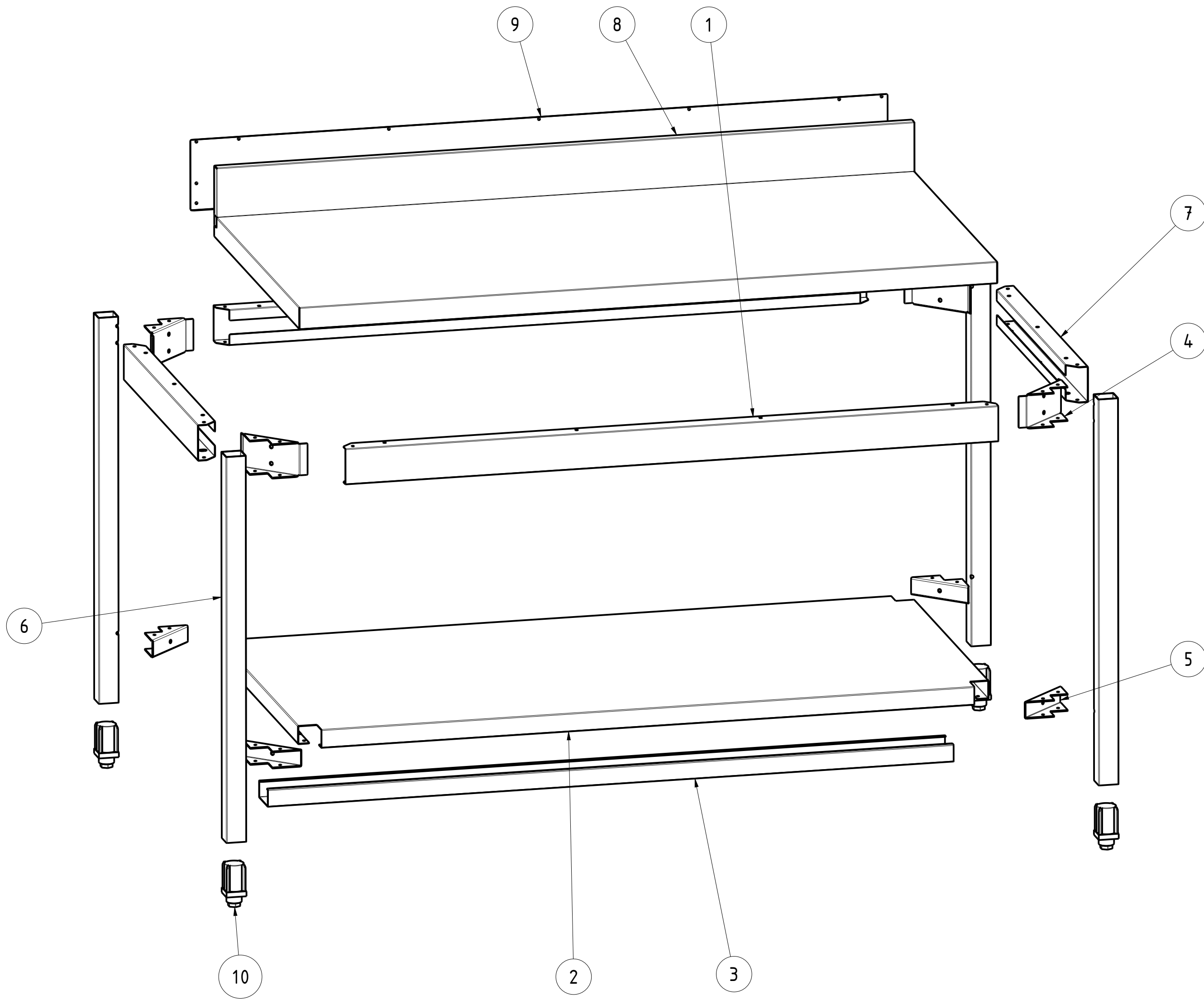
EXPLODED VIEW 3:20
