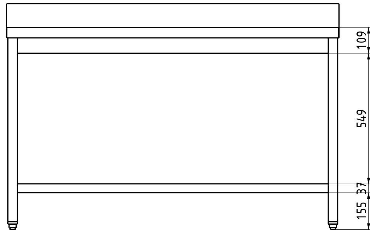
FRONT VIEW 1:10
