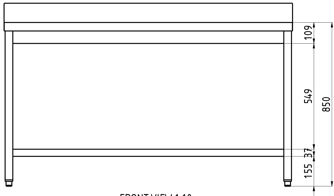
FRONT VIEW 1:10
