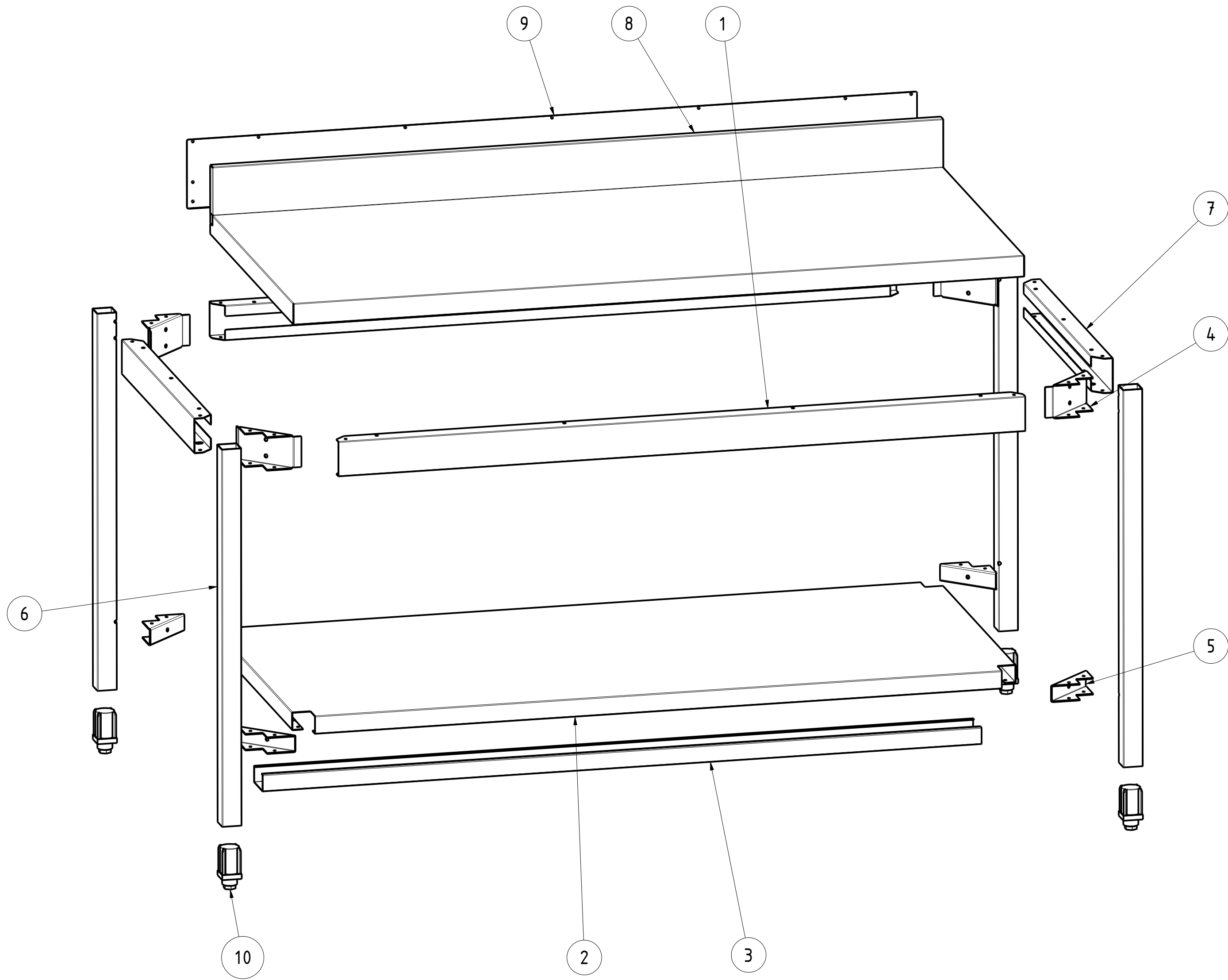
EXPLODED VIEW 3:20
