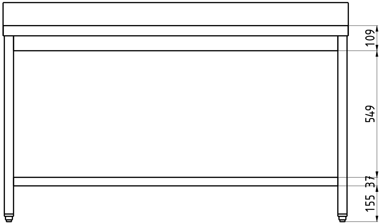
FRONT VIEW 1:10
