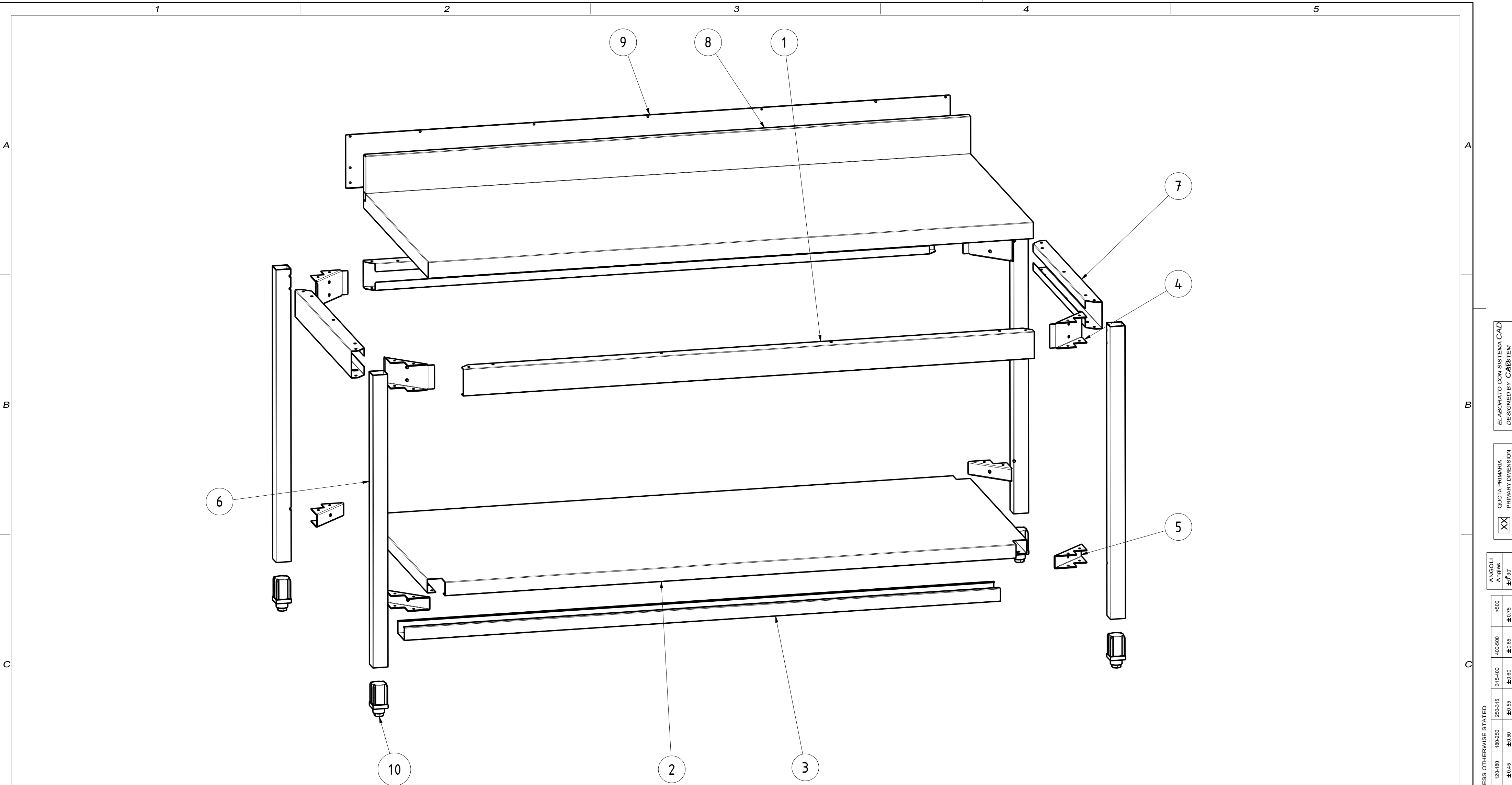
EXPLODED VIEW 3:20
