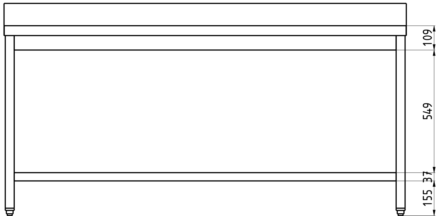
FRONT VIEW 1:10
