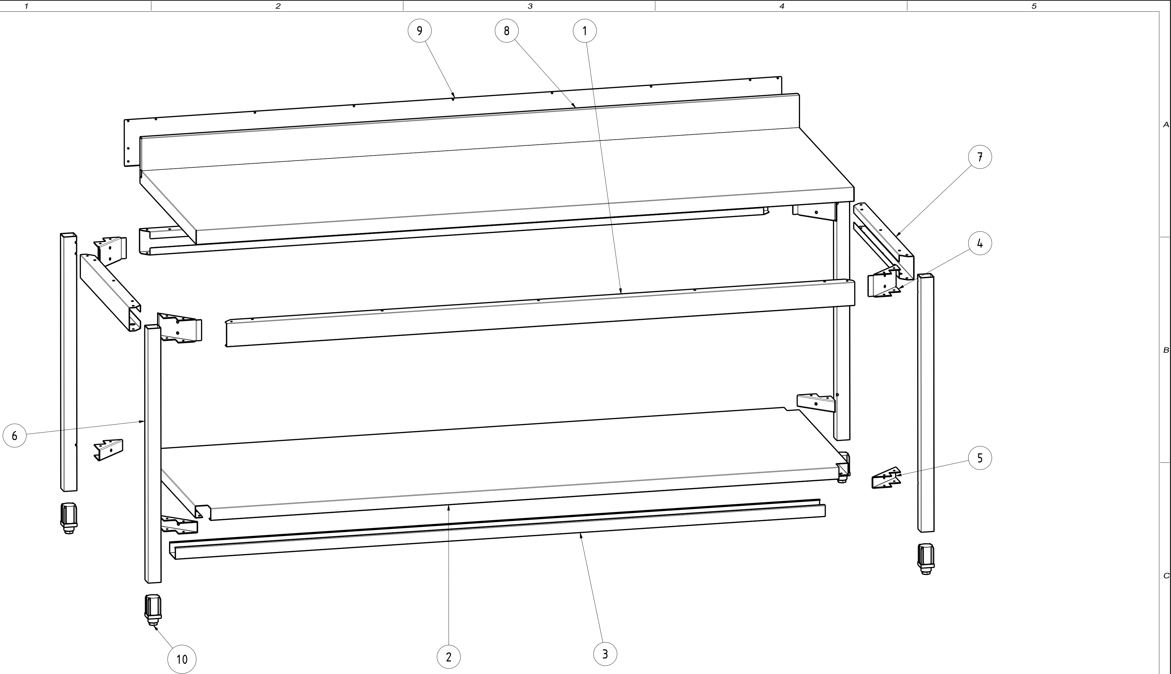
EXPLODED VIEW 3:20
