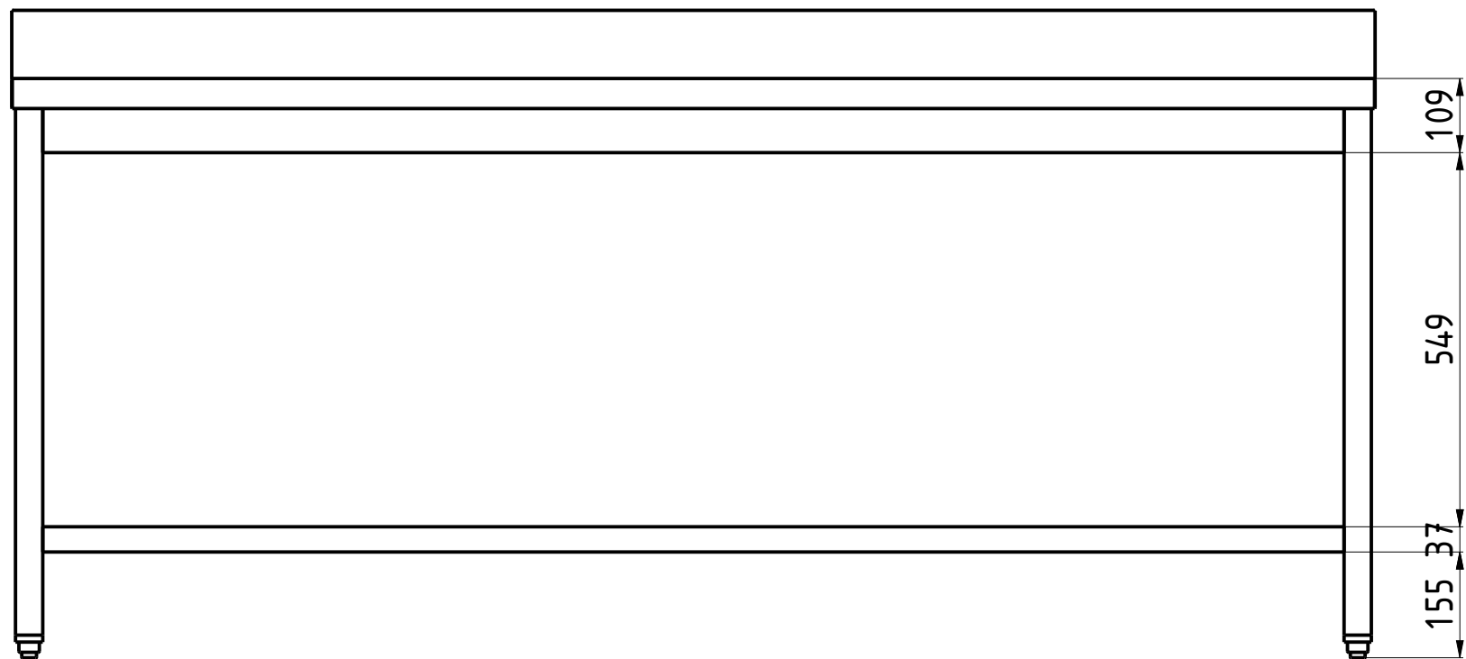
FRONT VIEW 1:10
