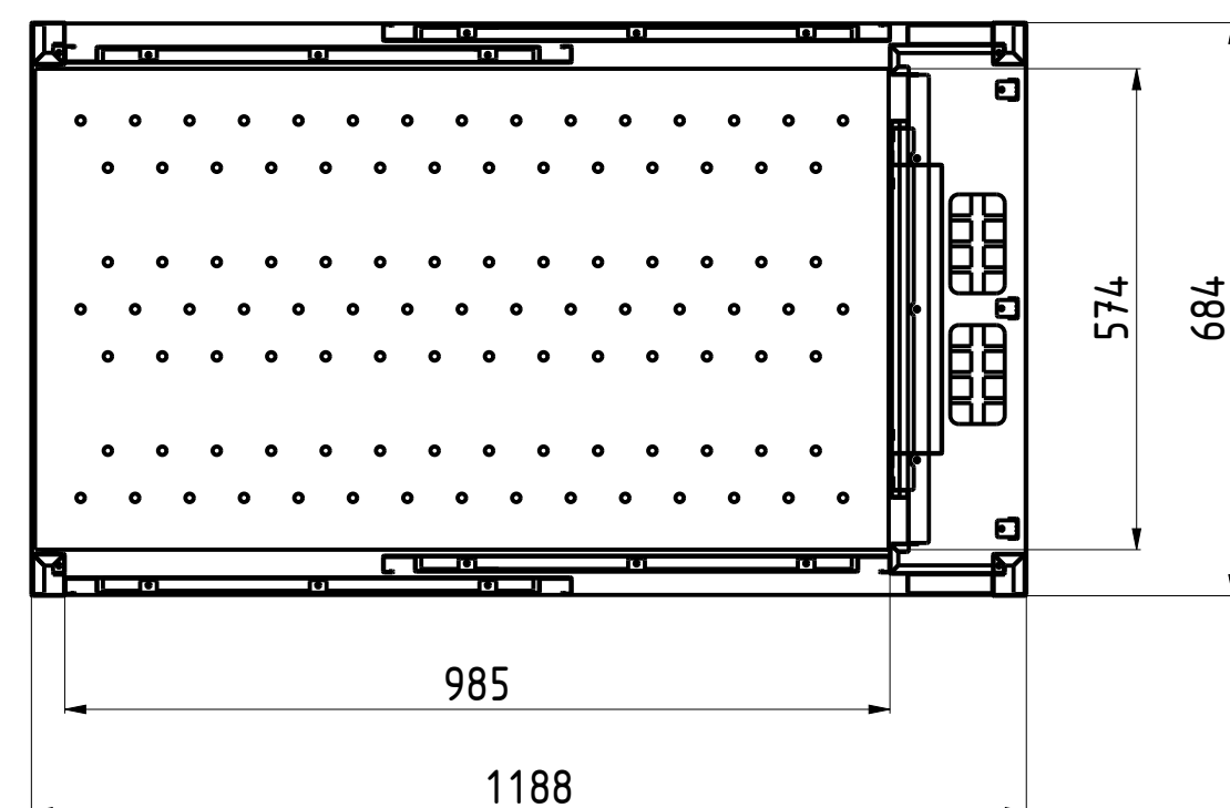
INTERNAL DIM C-C
