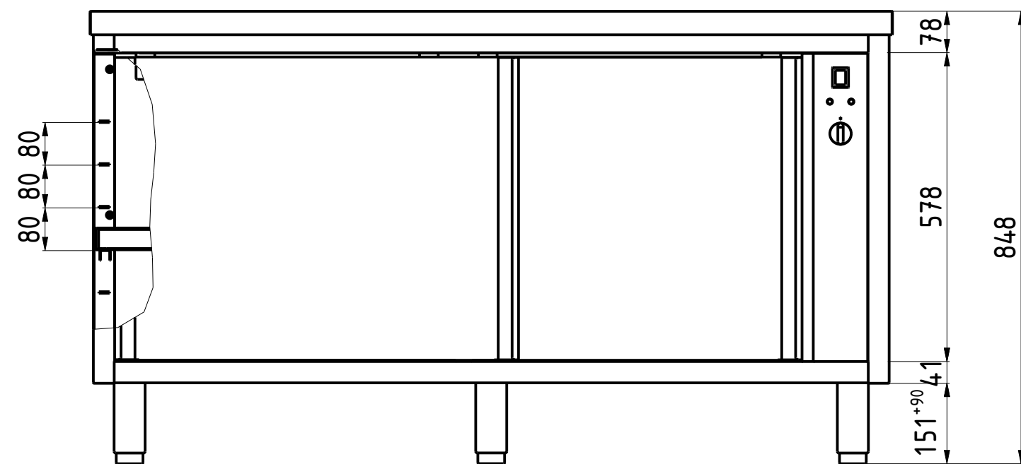
FRONT VIEW B-B 1:10
