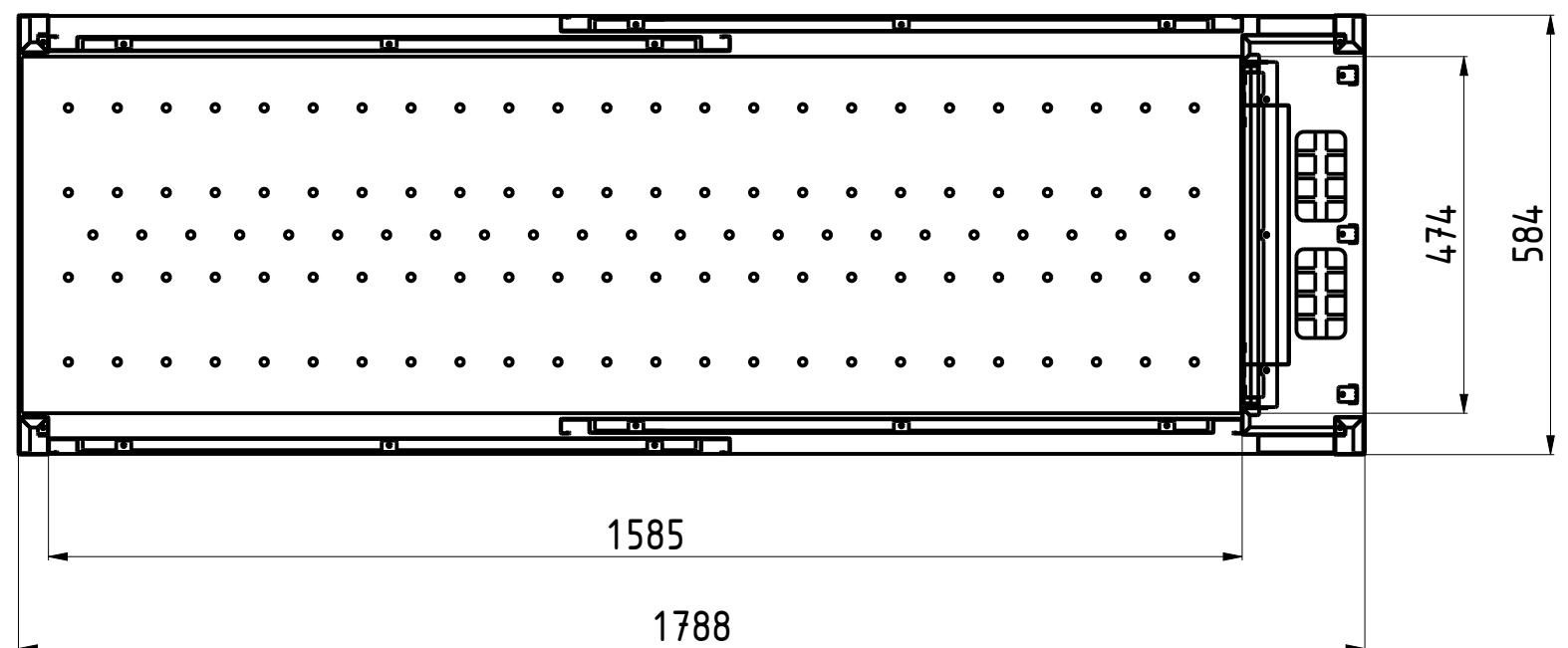
INTERNAL DIM C-C
