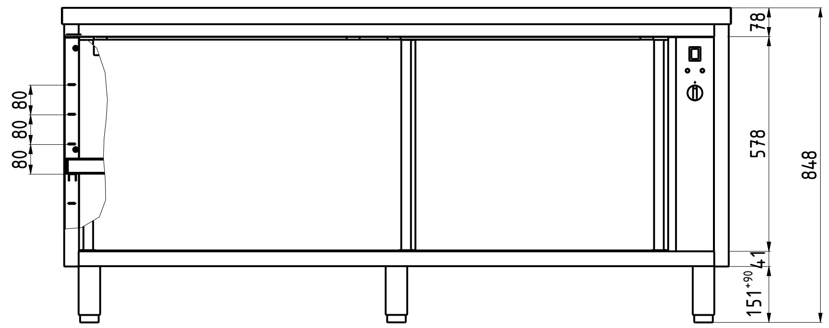
FRONT VIEW B-B 1:10
