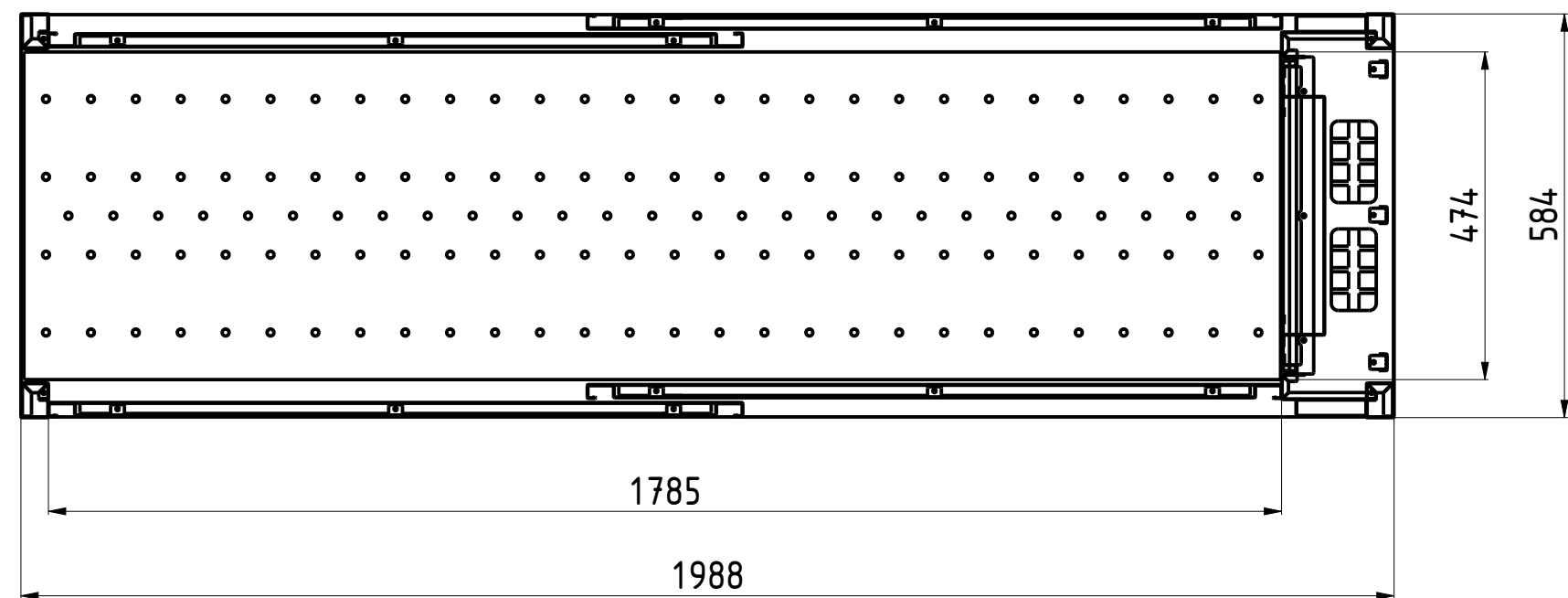
INTERNAL DIM C-C
