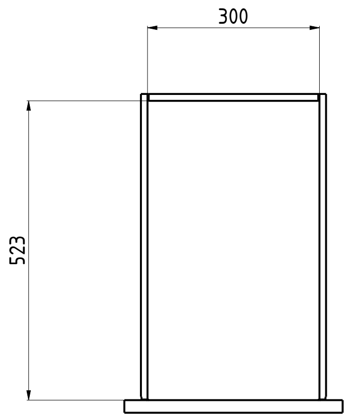
DRAWER 3:20
