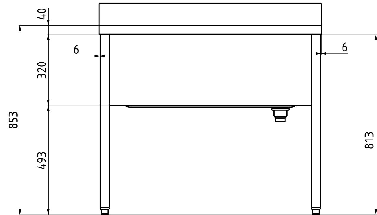
FRONT VIEW 1:10
