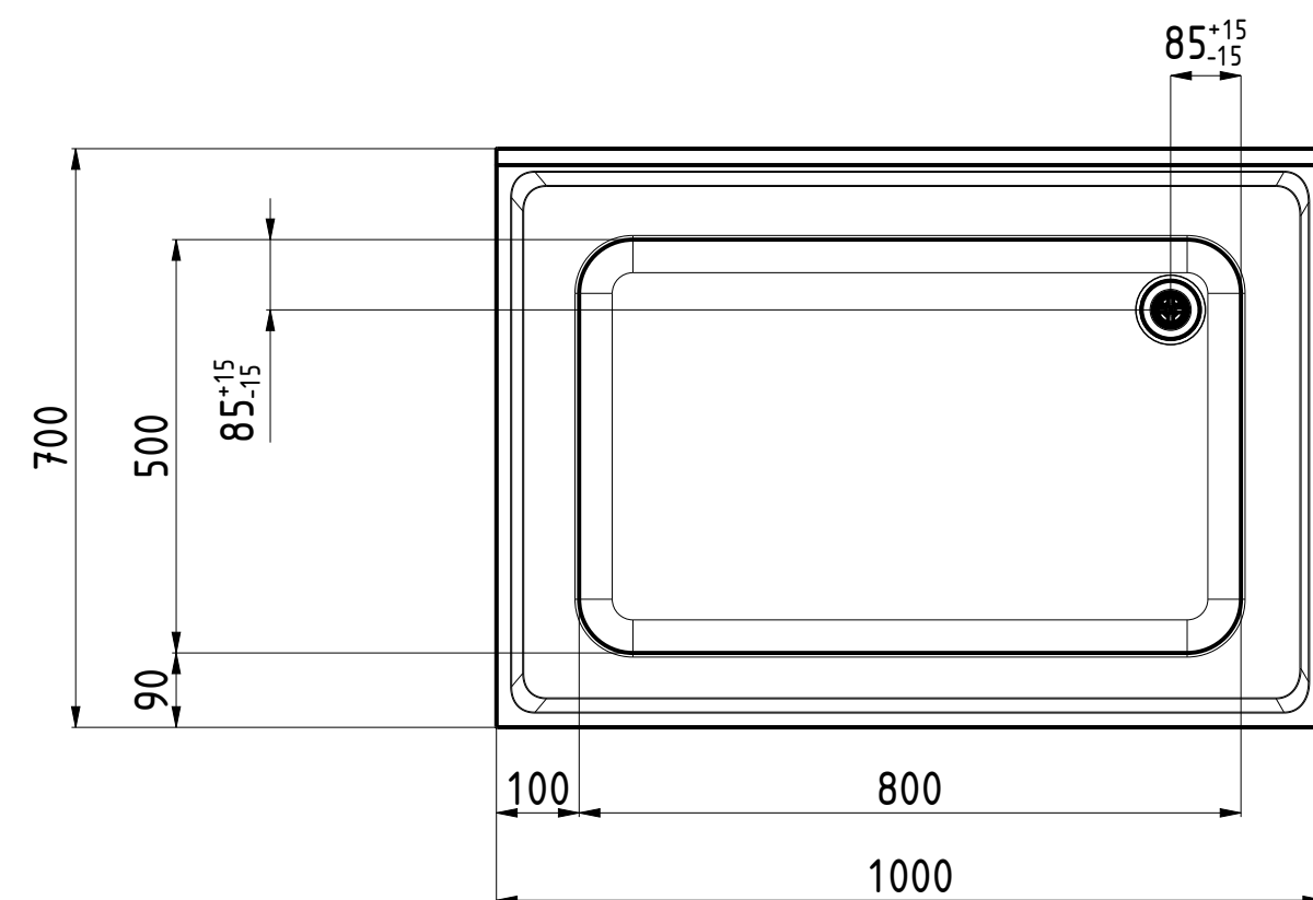
FRONT VIEW 1:10
