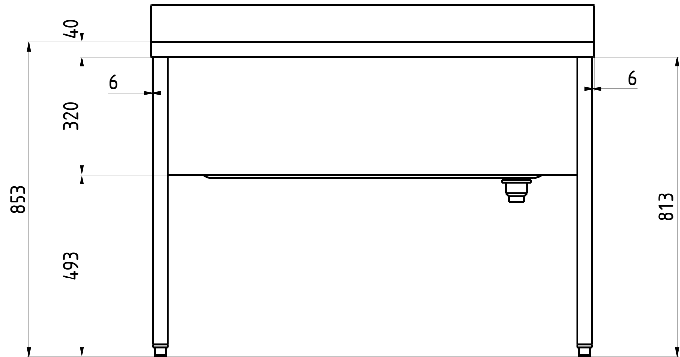
FRONT VIEW 1:10
