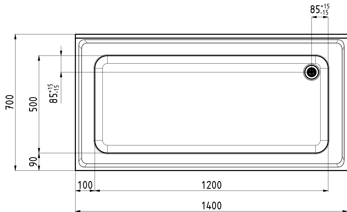
FRONT VIEW 1:10
