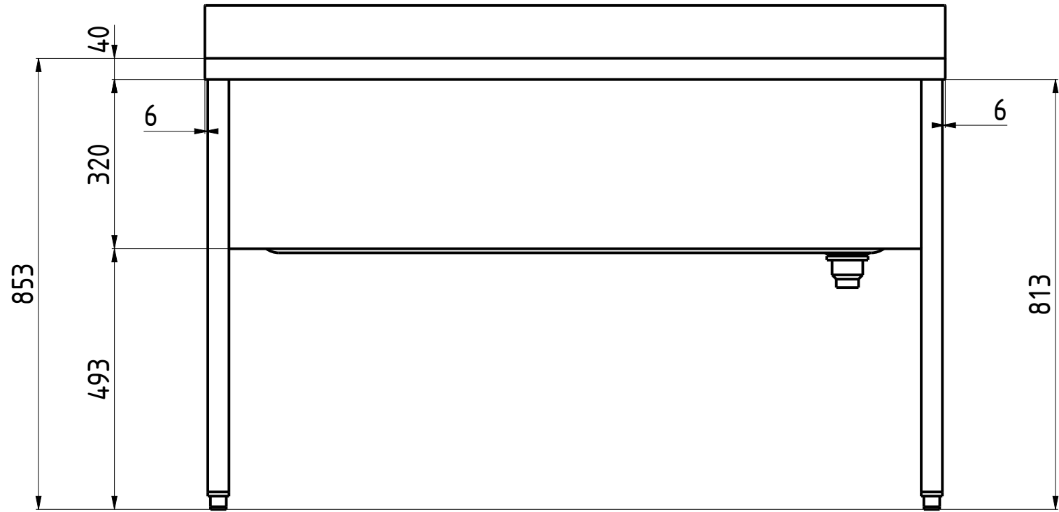
FRONT VIEW 1:10
