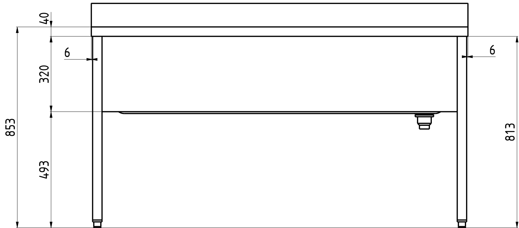
FRONT VIEW 1:10
