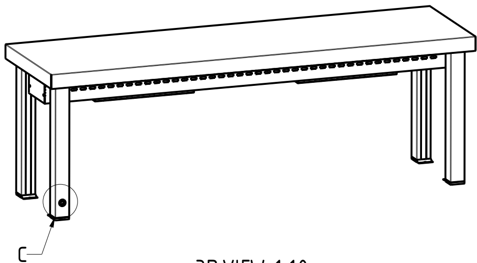
3D VIEW 1:10
