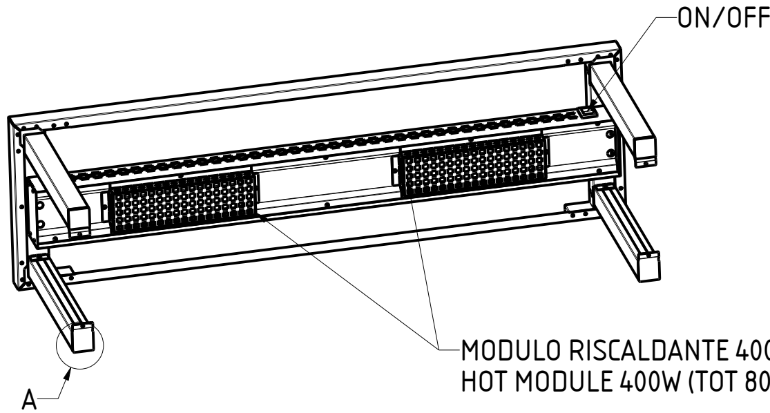
3D BOTTOM VIEW 1:10
