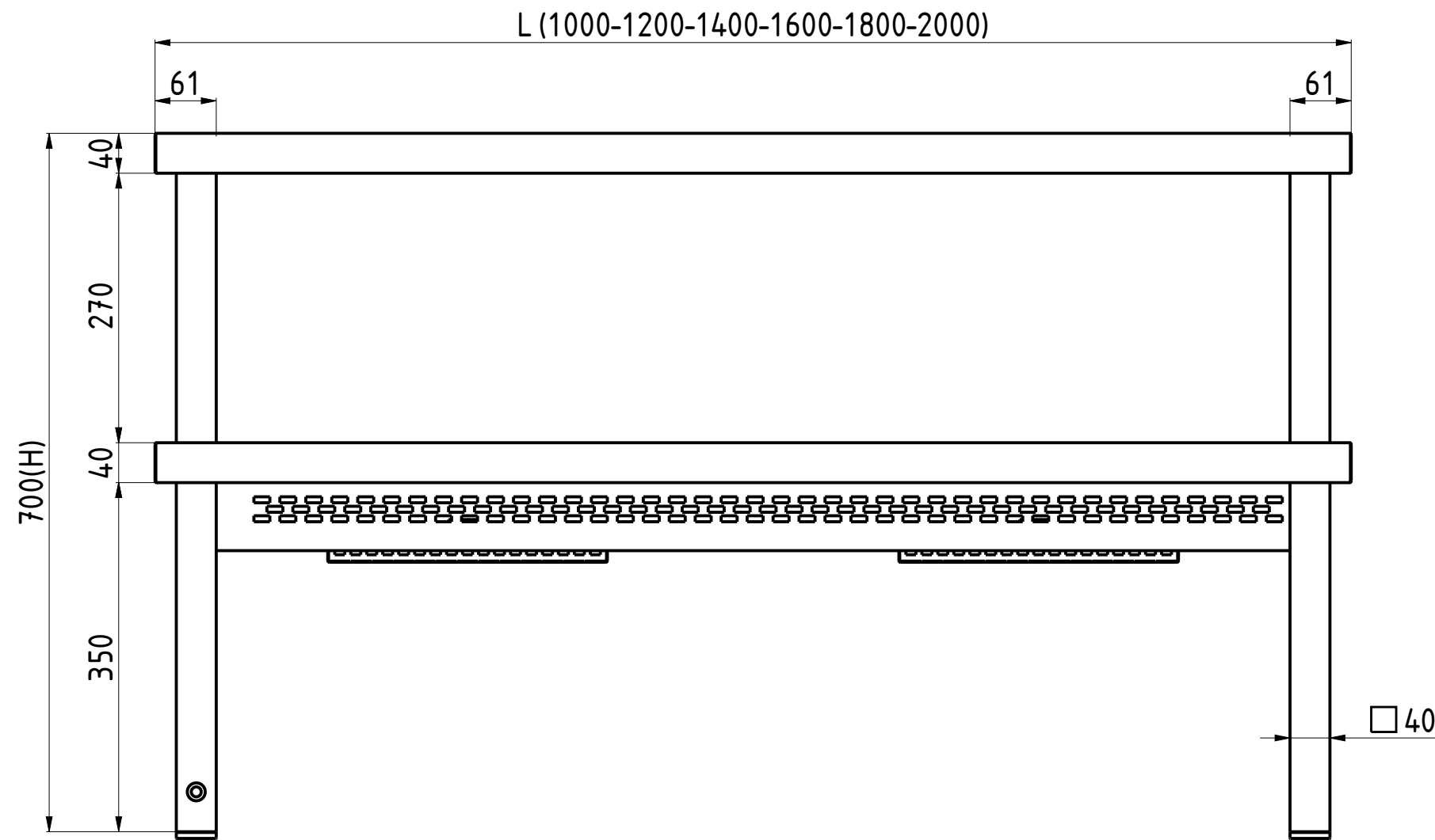
FRONT VIEW 1:6
