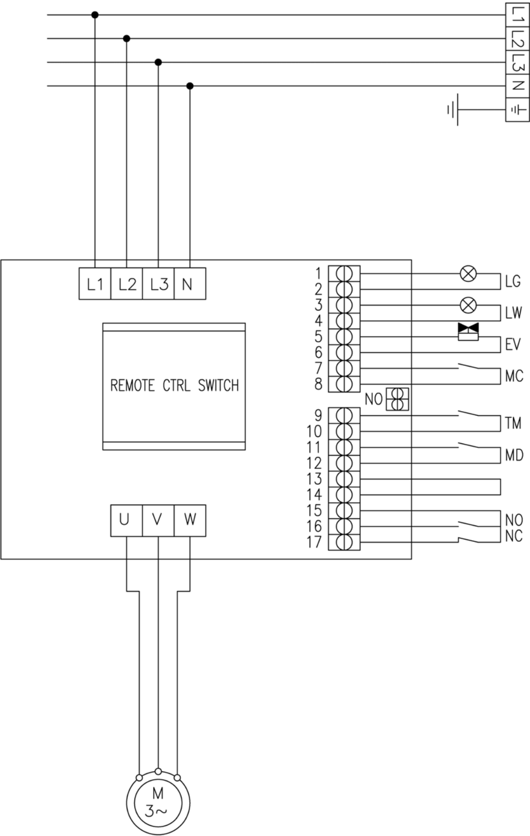
PPN-LCN-PPF-LCF10-18 / PPN-PPF25 (3 Phase)
