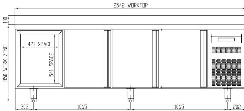
WORKTOP WITH UPSTAND
