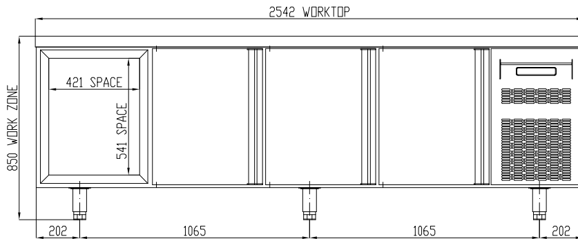
NO UPSTAND WORKTOP
