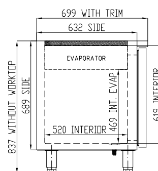
WITHOUT WORKTOP
