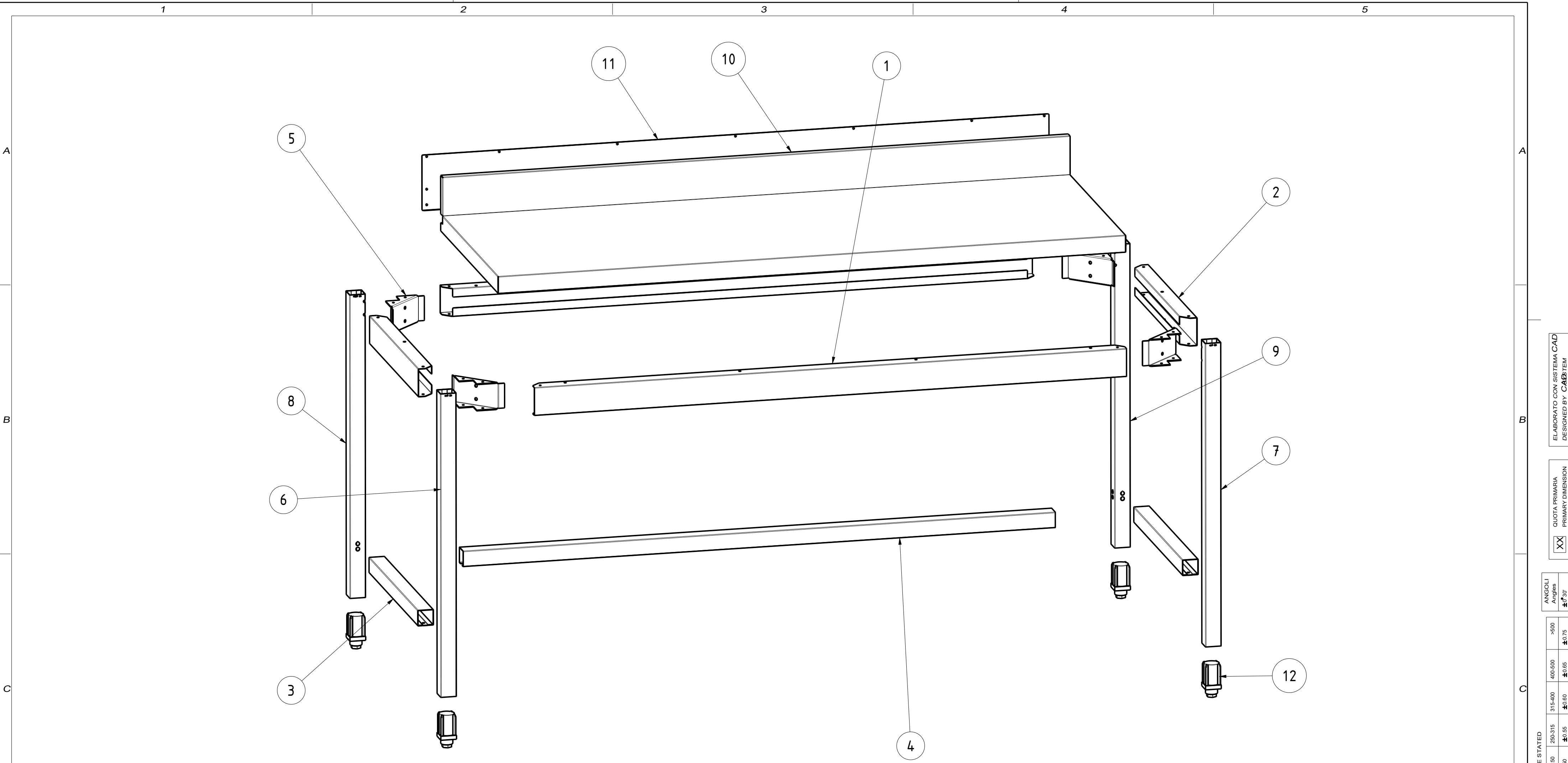
EXPLODED VIEW 3:20
