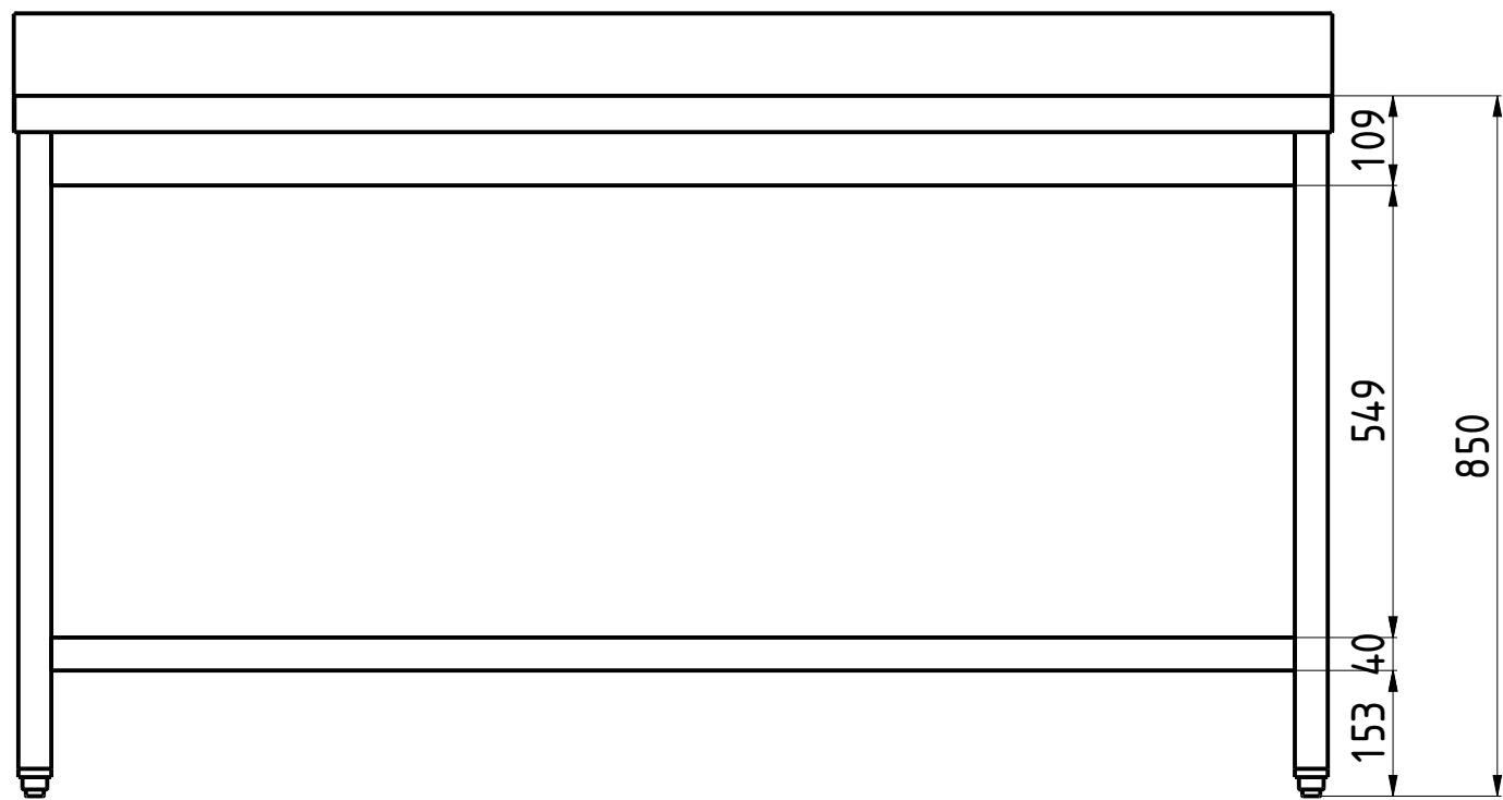
FRONT VIEW 1:10
