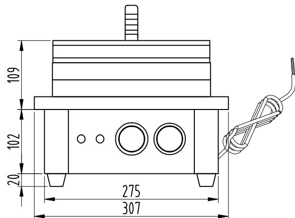
1- Front view
