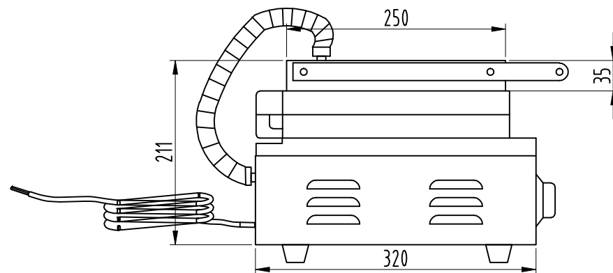
2- Side view
