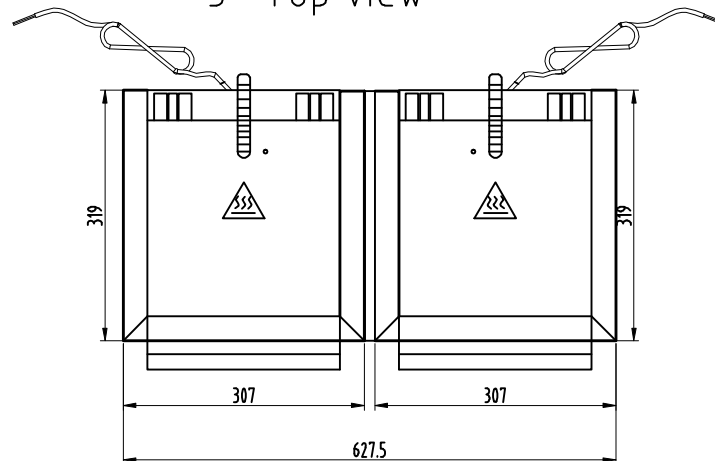
3- Top view
