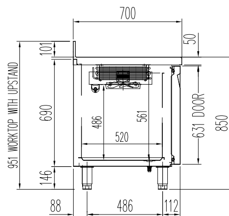
WORKTOP WITH UPSTAND
